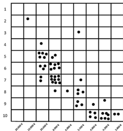
Young Cluster (<100 million years)
