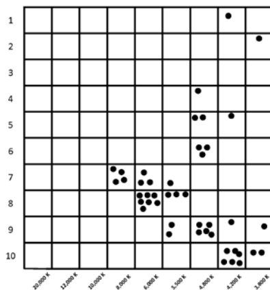
Middle-Age Cluster (100 million – 3 billion years)
