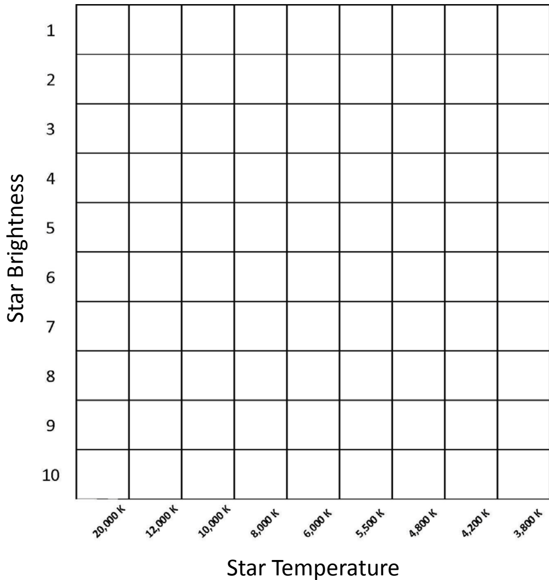
Middle-Age Cluster (100 million – 3 billion years)
