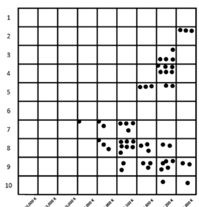
Old Cluster (> 3 billion years)
